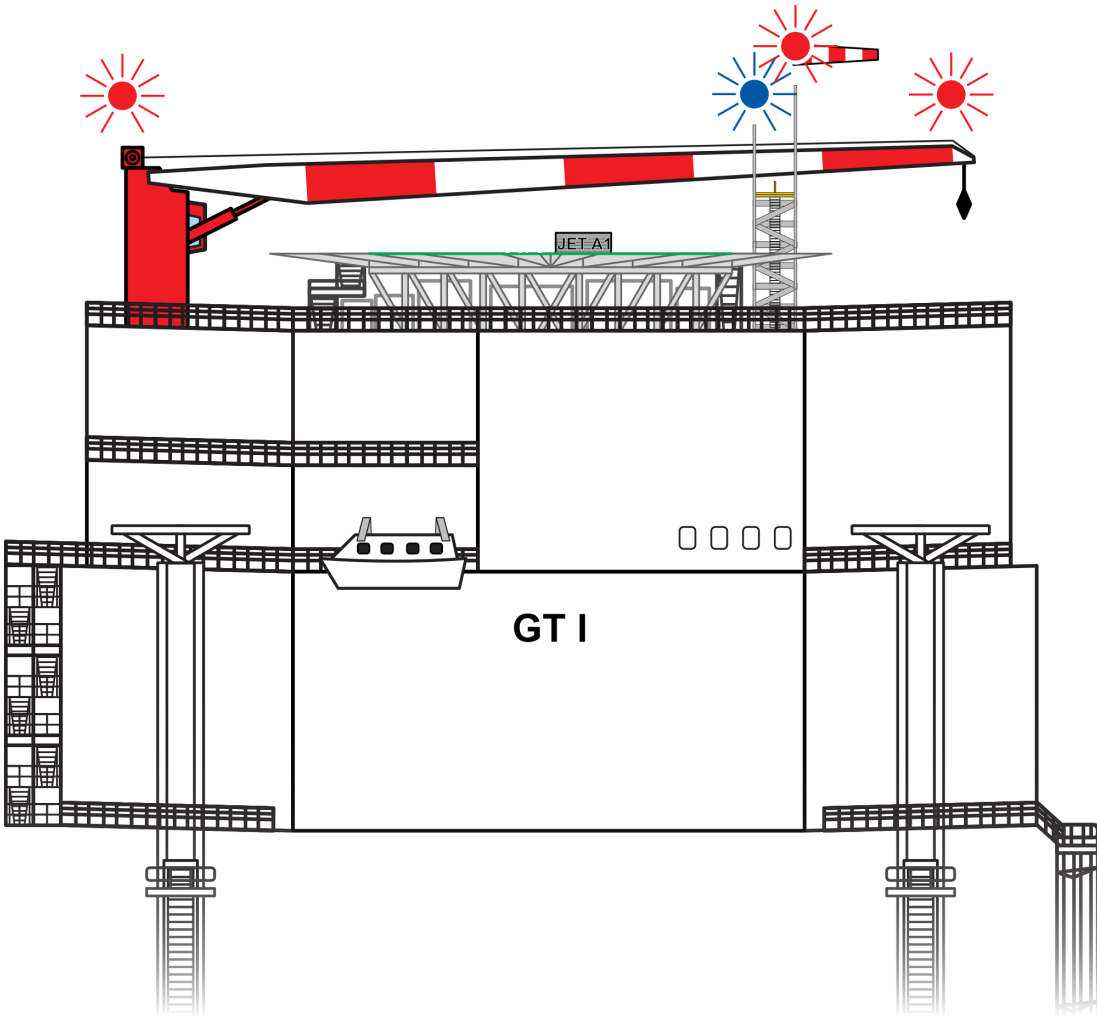
INSTALLATION PROFILE VIEW (NORTH)
